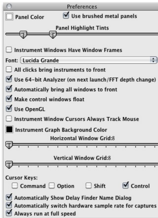
Figure 11.1: Main Preferences
