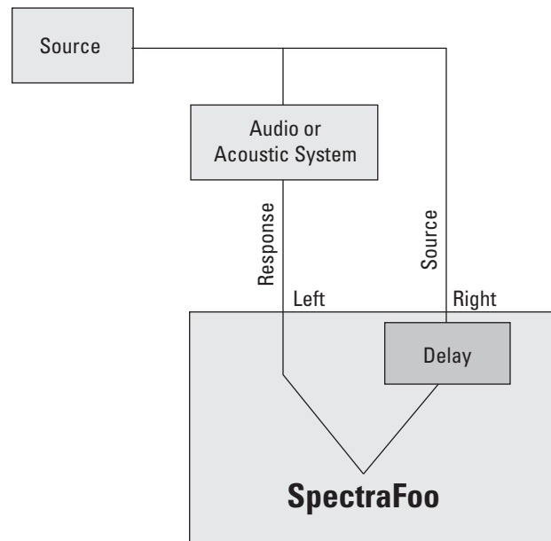
Figure 4.1: SpectraFoo Signal Arrangement for MBM Transfer Function
