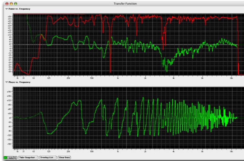
Figure 4.19: Transfer function without delay compensation
