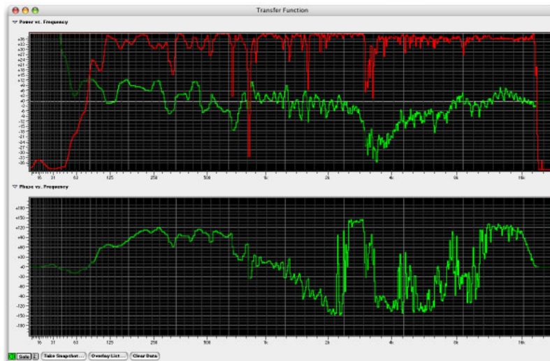
Figure 4.32: Sample transfer function
