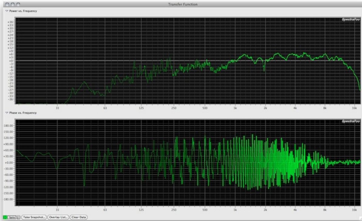
Figure 4.2: Transfer Function of a Room Response with a time delay
