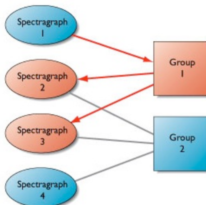
Figure 7.5: Parameter Passing
