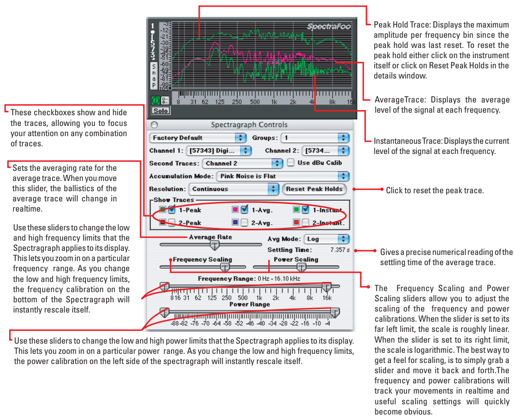
Figure 3.8: The Spectragraph and controls
