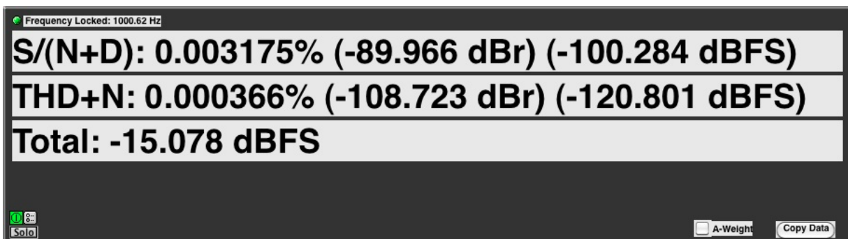
Figure 3.70: THD Meter
