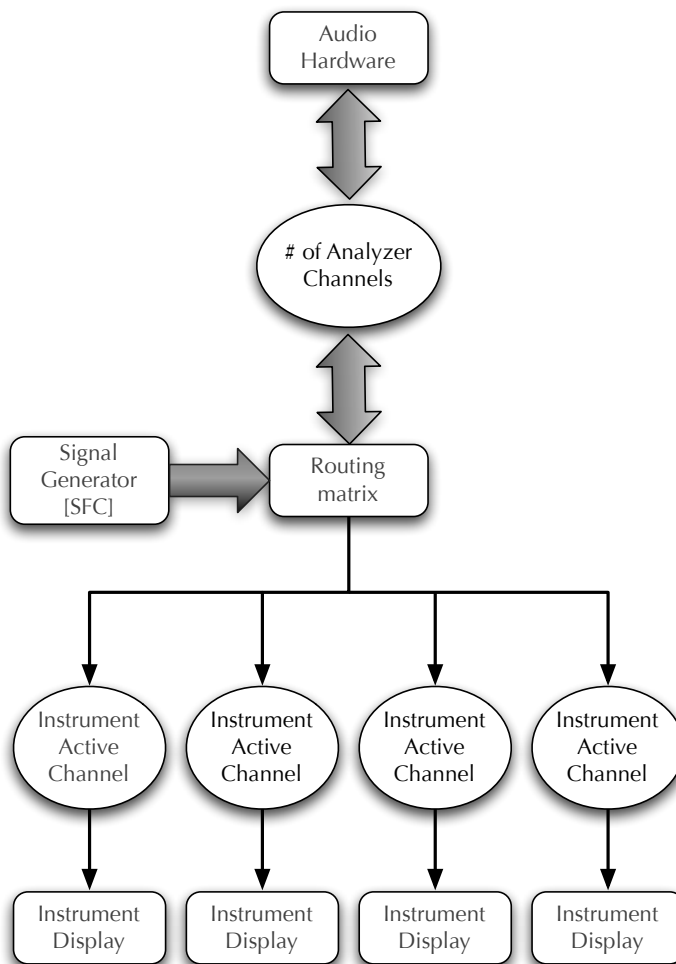
Figure 5.6: Analyzer channel routing
